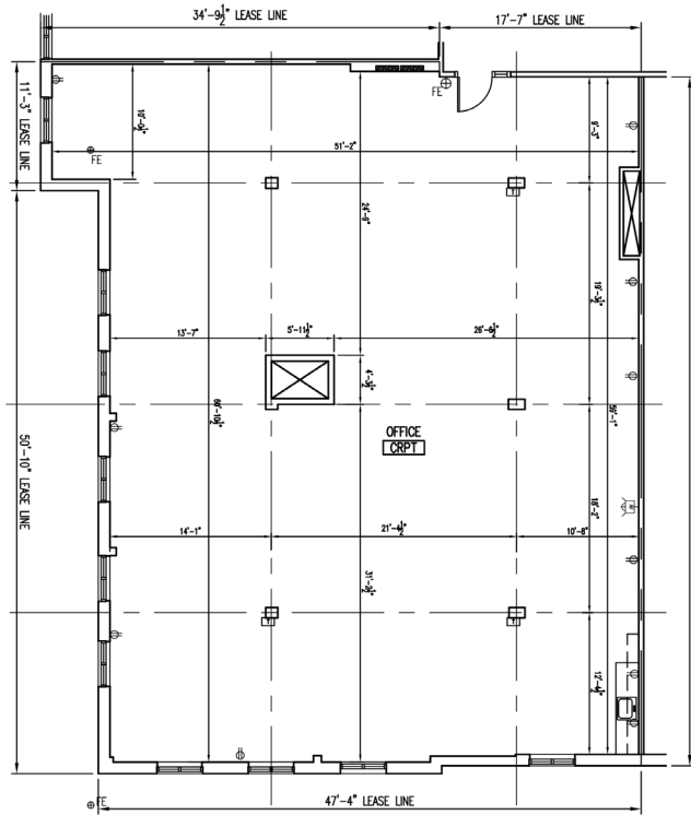
FLOOR PLAN SCALE: 3/32" = 1'-0"
