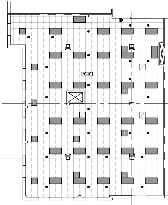
CEILING PLAN SCALE: 3/32" = 1'-0"
