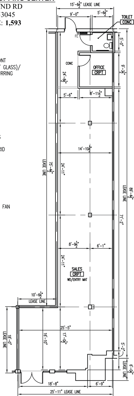
FLOOR PLAN SCALE: 3/32" = 1'-0"
